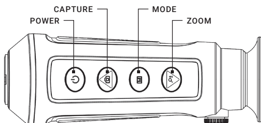
FIGURE 2-2. CONTROL BUTTONS
